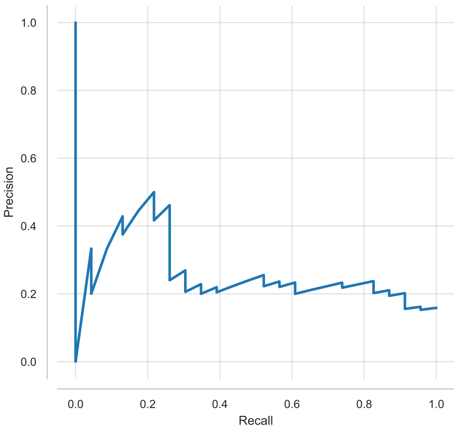
Precision-Recall Curve - LR
